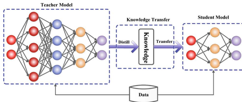
Fig. 2 The generic teacher-student framework for knowledge distillation
